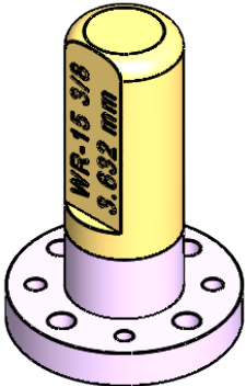
WR-15 WAVEGUIDE OFFSET
